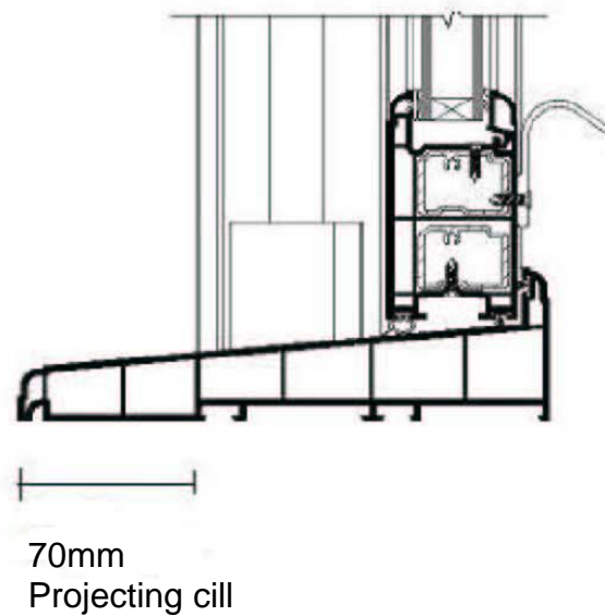
Vertical Slider with 210mm cill
